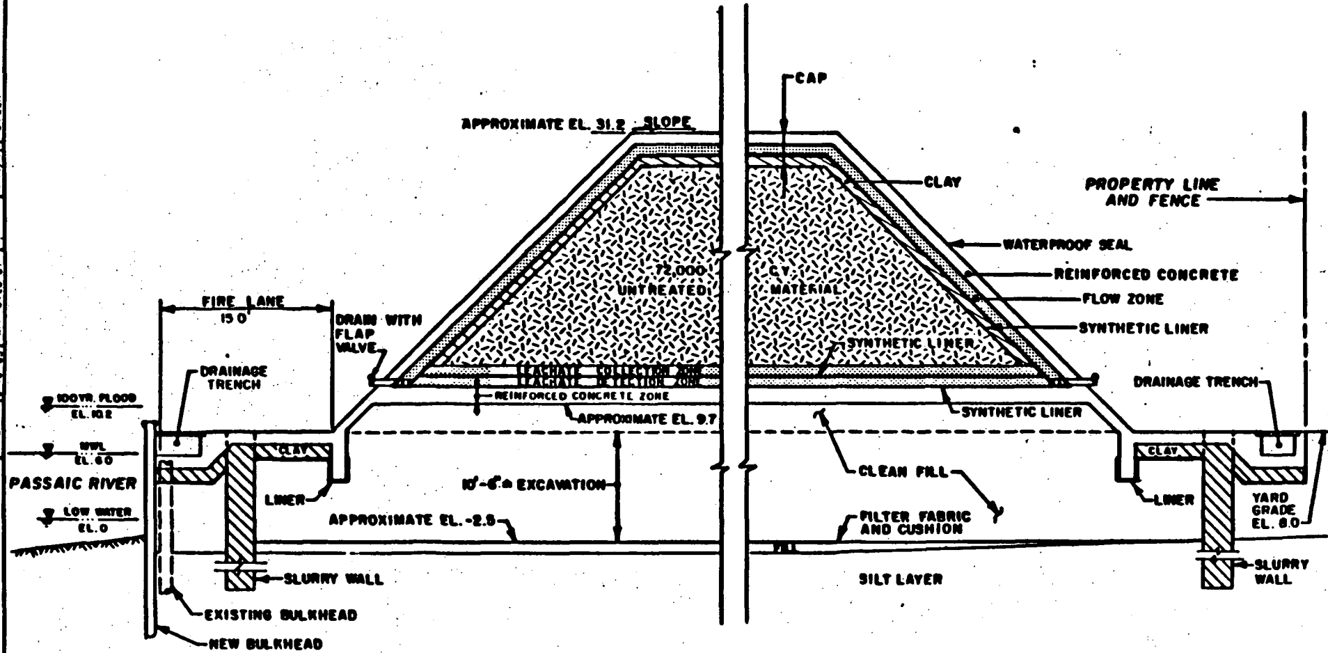
FIGURE 11 CONCEPTUAL CROSS SECTION LOOKING EAST ALTERNATIVE 5 80 LISTER AVENUE PREPARED FOR DIAMOND SHANROCK DALLAS, TEXAS
