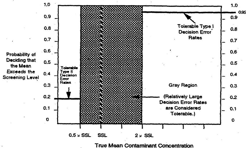
Figure 5. Design performance goal diagram.
